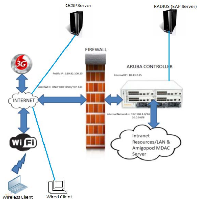
Figure 110 VIA Topology
